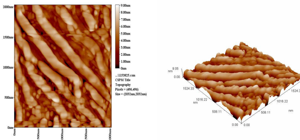
b- \text{Cd}_{0.98}\text{Cr}_{0.02}\text{O}
